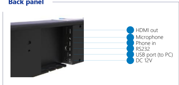
Back panel
